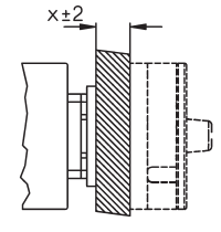
Mounting hole Mounting screw: S3631N M=1,2-1,4 Nm
