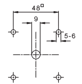
Mounting hole Mounting screw: S3631N M=1,2-1,4 Nm
