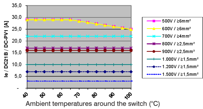
Switch open LSA(O)16 ..., 2 contacts in series + 2 parallel (A2+2)
