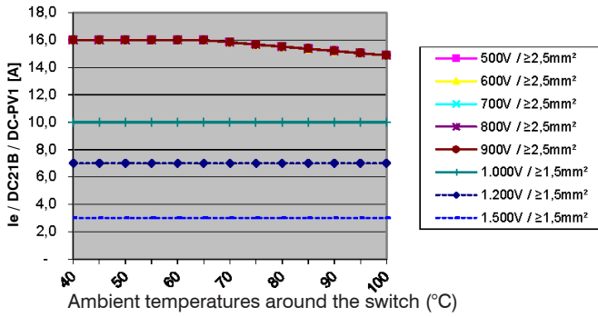
Switch open LSA(O)16..., 2 contacts in series (A2)
