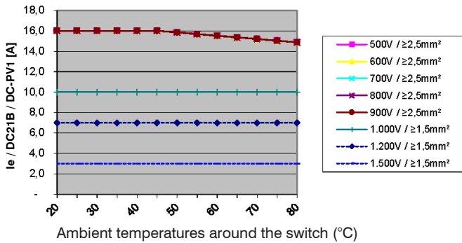
Switch enclosed LSA(O)16 PFL..., 2 contacts in series (A2)
